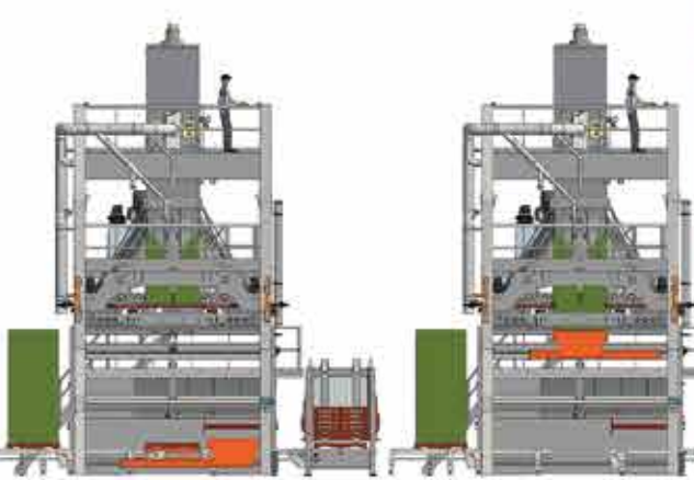
1 Bale leaves compression chute and is placed on the lift plate
